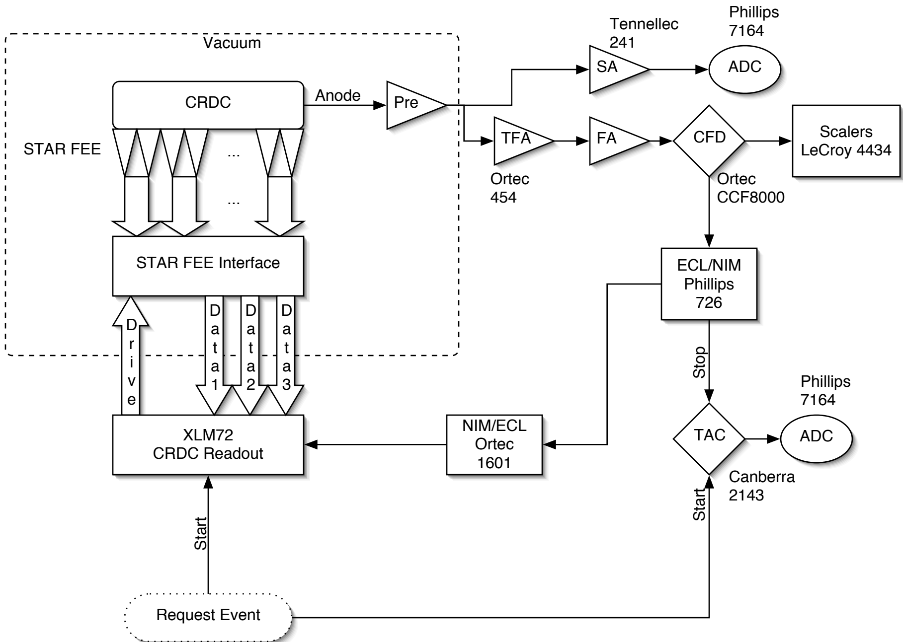
CRDC Electronics Diagram
