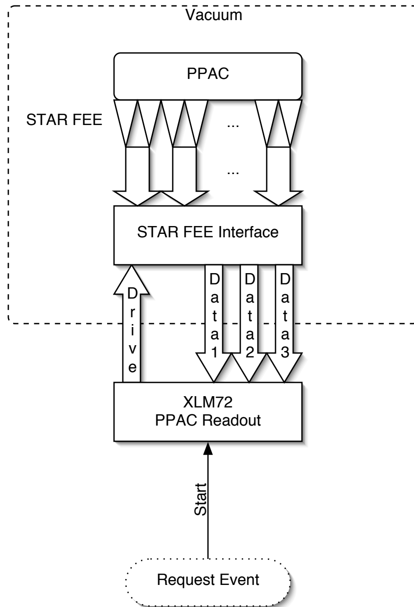
Tracking PPAC Electronics Diagram
