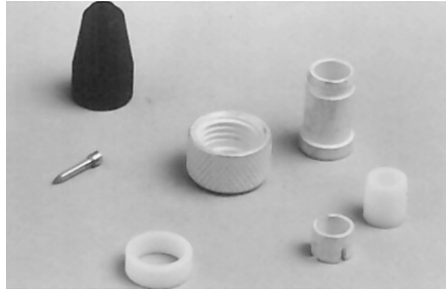
C-22 Microdot Male Plug for Miniature 100-Ω Cable
