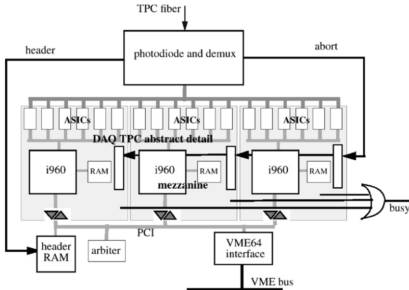
Fig. 1. Block diagram of the TPC, SVT and FTFC RBs.
