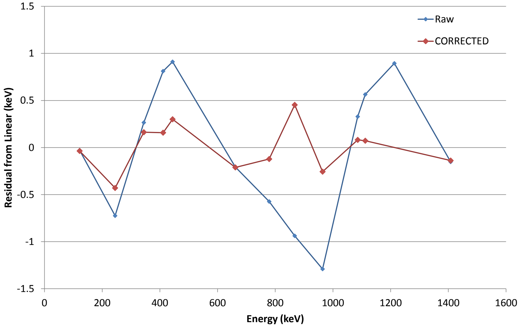
10MeV CC (Crystal 28) w/ and w/o INL Correction
