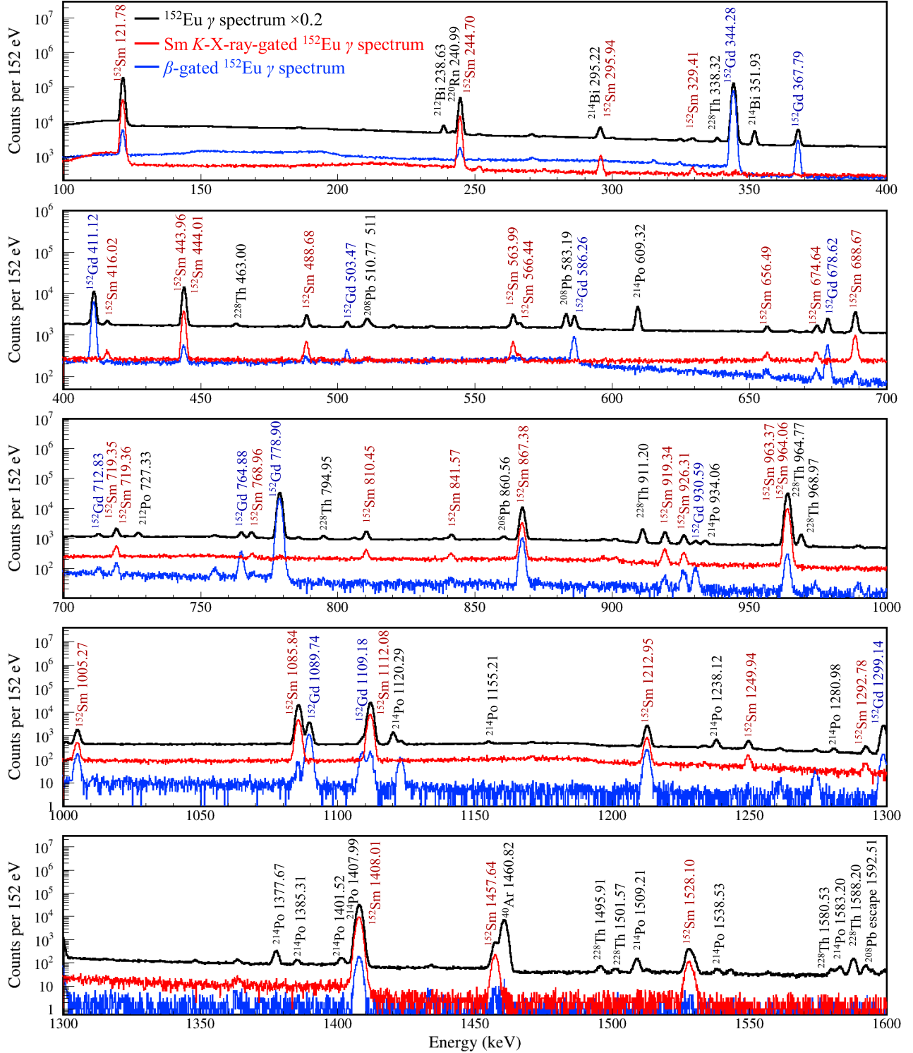
FIG. 13. Black represents the raw \gamma -ray spectrum measured by XtRa1 using the ^{152}\text{Eu} source placed at the center of the chamber. Red represents the XtRa1 \gamma -ray spectrum gated by the Sm K_{\alpha} and K_{\beta} X rays measured by LEGe. Blue represents the XtRa1 \gamma -ray spectrum gated by the electrons measured by MSD26. The raw spectrum is scaled down by a factor of 5 for better comparison.
