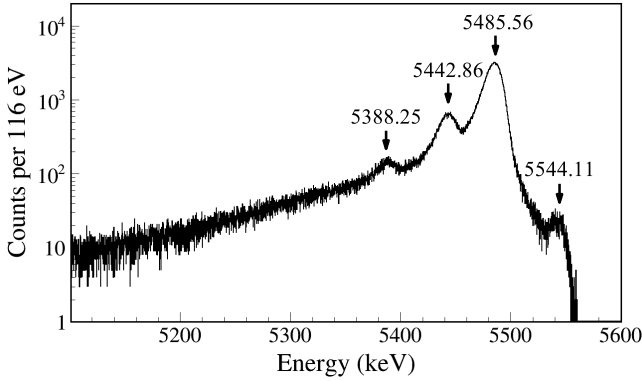
FIG. 10. \alpha spectrum measured by MSD26 using the ^{241}\text{Am} source. The \alpha energy values are adopted from Ref. [80] rounded to the nearest 0.01 keV. An EMG fit of the main peak yields a FWHM of 17.0 keV, corresponding to an energy resolution of 0.31%.
