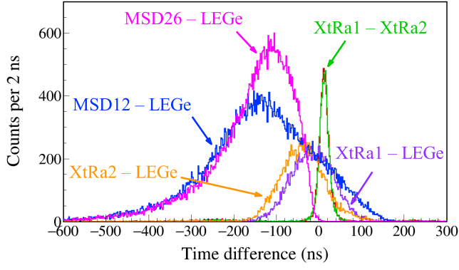
FIG. 14. Coincidence time spectra between each detector obtained using the ^{60}\text{Co} 1173-keV and 1332-keV \gamma - \gamma coincidences, ^{152}\text{Eu} 40–46-keV and 1408-keV X- \gamma coincidences, and ^{241}\text{Am} 5486-keV and 59.5-keV \alpha - \gamma coincidences.
