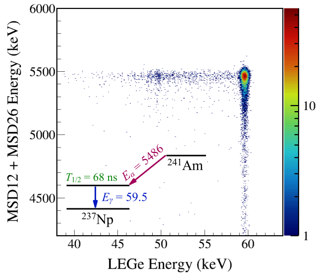
FIG. 12. Coincidence spectrum between the MSD detector telescope and LEGe obtained using the ^{241}\text{Am} source placed at the center of the chamber. A simplified ^{241}\text{Am} decay scheme shows the dominant \alpha - \gamma sequence.
