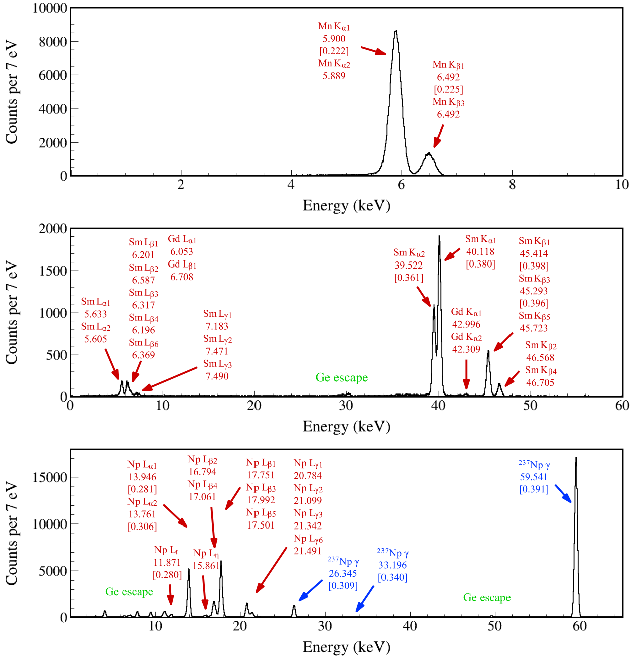
FIG. 7. X-ray and/or \gamma -ray spectra measured by the LEGe detector using the ^{55}\text{Fe} (top), ^{152}\text{Eu} (middle), and ^{241}\text{Am} (bottom) sources. All the X-ray energy values are adopted from Ref. [70] rounded to the nearest 0.01 keV. All the \gamma -ray energy values are adopted from Ref. [72] rounded to the nearest 0.01 keV. The FWHM values used to characterize the energy resolution of LEGe are indicated within brackets.
