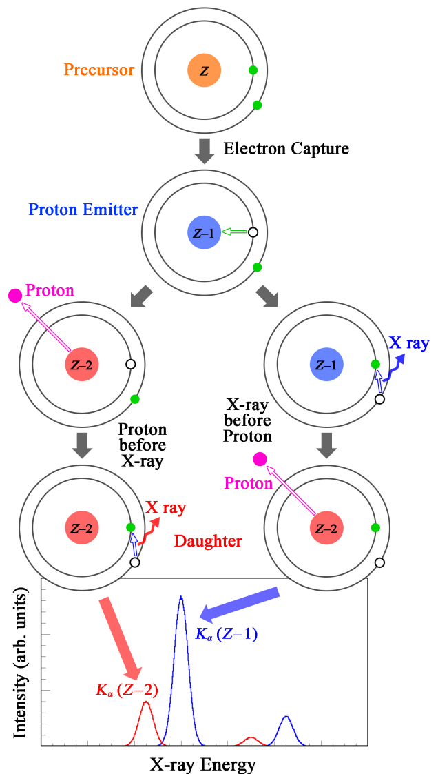
FIG. 3. Schematic illustrating the Particle-X-ray Coincidence Technique. See text for details.
