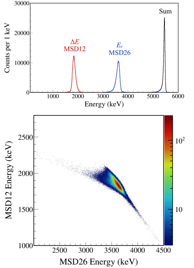
FIG. 11. Upper: ^{241}\text{Am} \alpha -energy spectra measured by MSD12 (energy-loss) and MSD26 (residual energy). An EMG fit of the energy-sum peak yields a FWHM of 52.1 keV, corresponding to an energy resolution of 0.95%. Lower: \Delta E - E 2D plot.
