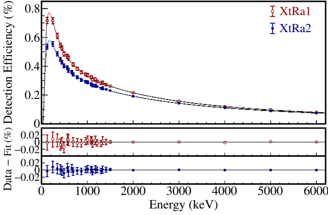
FIG. 9. Absolute \gamma -ray photopeak detection efficiency of the two XtRa detectors obtained using the ^{152}\text{Eu} , ^{137}\text{Cs} , and ^{60}\text{Co} sources placed at the center of the chamber. The ^{137}\text{Cs} data point at 662 keV is only applicable to XtRa2 due to the source placement. The 6 data points above 1500 keV are GEANT4 simulated efficiencies scaled by a factor to match the low-energy source data. The efficiency curves are generated by fitting all measured and simulated data points.
